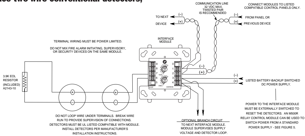
Figure 4. Interface two-wire conventional detectors, NFPA Style D:
