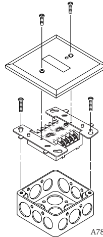
Figure 2A. Module mounting with barrier:
