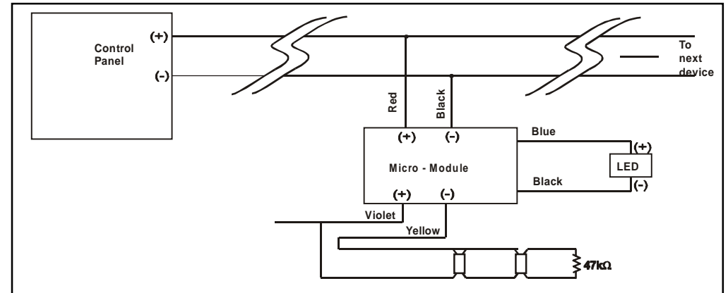
Figure 2. Wiring diagram for M503ME Monitor Module.
