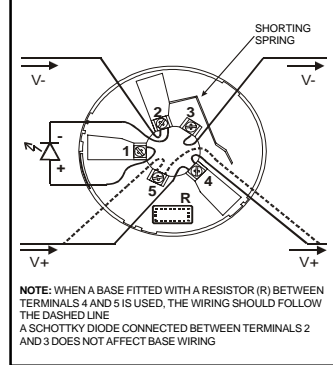
Figure 1: Base Terminal Wiring
