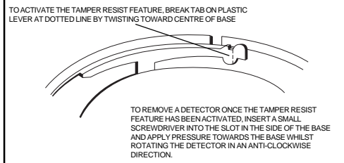
Figure 2: Tamper Resist Feature
