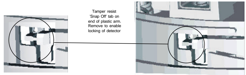
FIGURE 3 SECURING AND REMOVING DETECTOR HEAD FROM BASE
