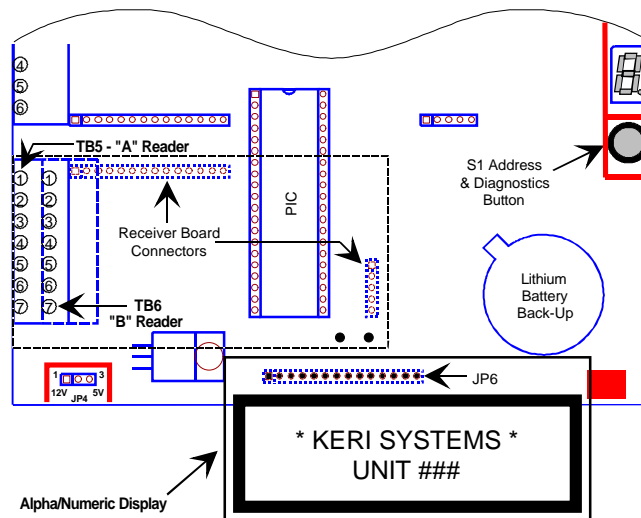
Figure 3 – Connecting the LCD-1 to the Controller
