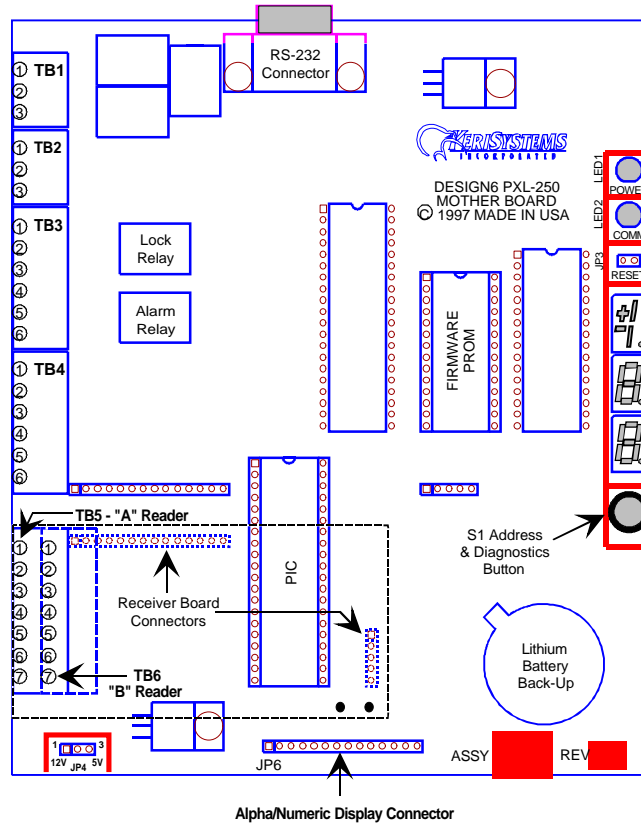
Figure 2 – Location of JP6 on the Controller
