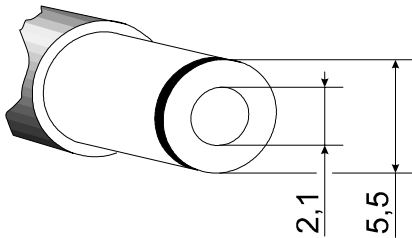
fig. 1 - output connector (all in mm)
